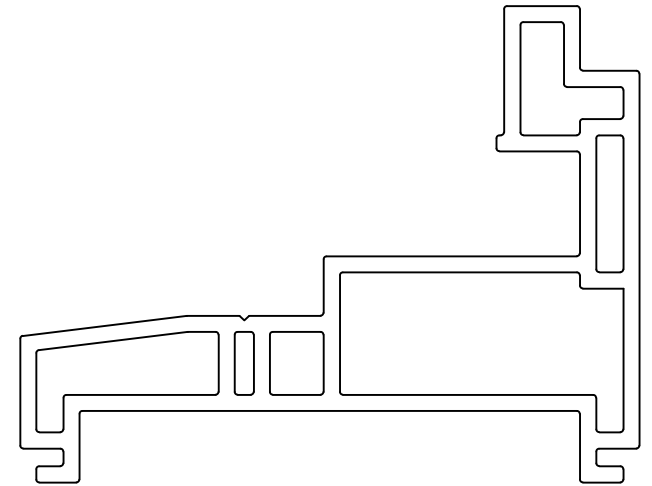
5012 CASEMENT MAIN FRAME WELDED
