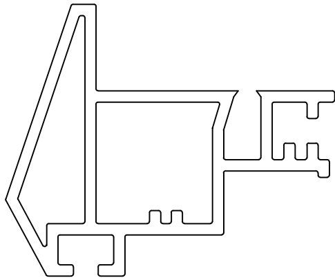
5000 CASEMENT SASH WELDED
