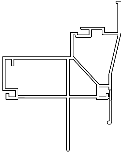
1511 PICTURE WINDOW MAIN FRAME w/ FIN & J WELDED
