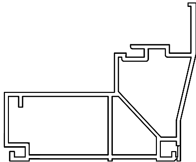
1011 PICTURE WINDOW MAIN FRAME NO FIN WELDED
