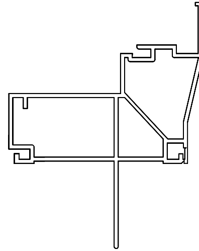
1611 PICTURE WINDOW MAIN FRAME w/ FIN WELDED
