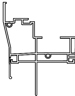
1512 NEW CONSTRUCTION SH JAMB w/ FIN & J
