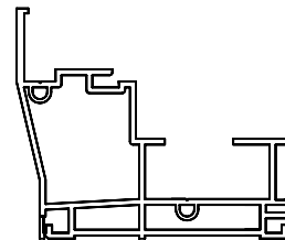
1012 NEW CONSTRUCTION SH JAMB NO FIN WELDED
