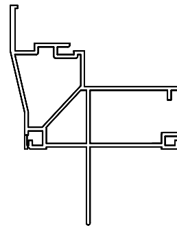
1611 NEW CONSTRUCTION SH HEAD w/ FIN
