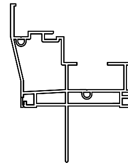
1612 NEW CONSTRUCTION SH JAMB w/ FIN
