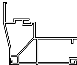
1011 NEW CONSTRUCTION SH HEAD NO FIN WELDED
